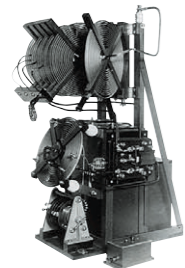
quenched spark radiotelegraph unit (1916)
