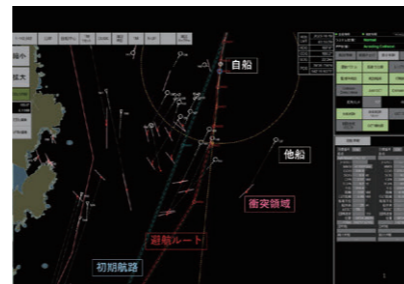
Collision avoidance route generation screen
