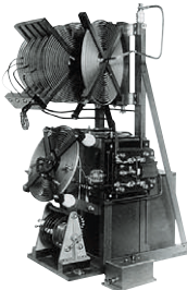
quenched spark radiotelegraph unit (1916)
