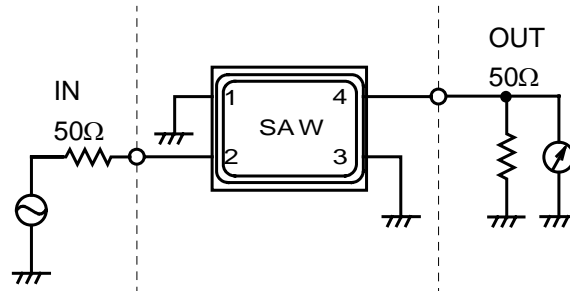
Fig.1 Measuring circuit 2.0±0.1
