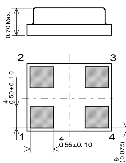
Fig.2 Package dimensions (in mm)
